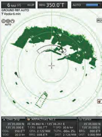
Simplified ARPA
